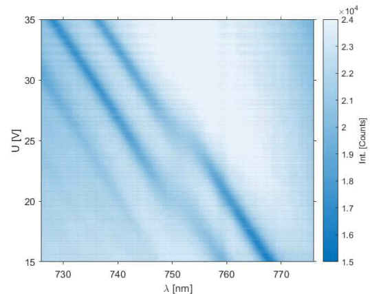
Figure 2: Reflectivity spectrum of the structure in Figure 1, Cavity is tuned over a range of ~1μm via piezo voltage
