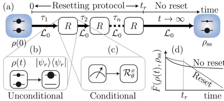
Fig. Illustration of stochastic resetting protocols and relaxation speedup. (a) For simplicity, we showcase a single qubit system, initialized in the state \rho(0) and evolving under a reset-free Liouvillian \mathcal{L}_0 . Times \tau_j elapsing between
