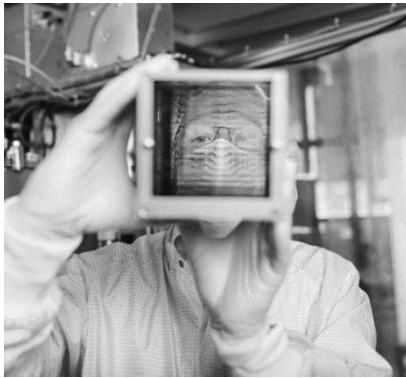
Fig. 1: Lobster-Eye telescope
